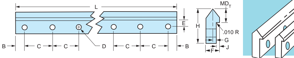
Standard Drilled Track Hole Spacing and Size
