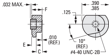
Fig. 6 REVER (No Screw Supplied - 1/2 Turn)
